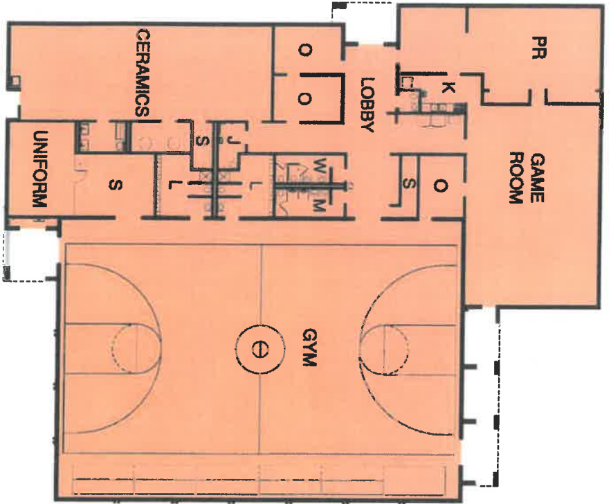
EXISTING FLOOR PLAN 1"=30'-0" EXISTING: 15,076 SF
